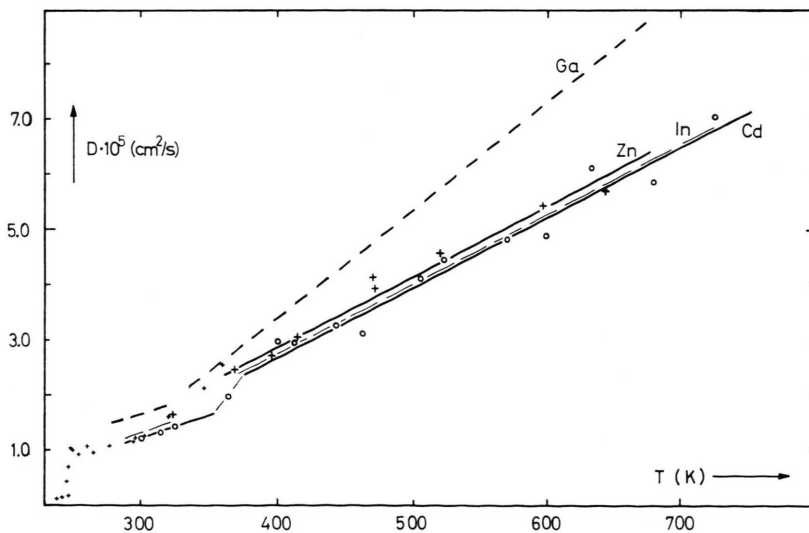
Fig. 1. Linear plot of D vs T for the diffusion coefficients of impurities in liquid Ga. Crosses: ^{65}\text{Zn} . Small crosses: ^{65}\text{Zn} from Ref. 5. Rings: ^{115}\text{Cd} . Line with short dashes: ^{72}\text{Ga} . Long dashes: ^{114}\text{In} .
